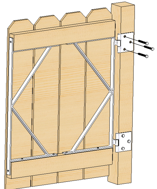
FIG. 3 SINGLE GATE
