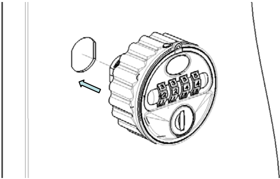
Figure 1. Position lock through door panel as shown.
