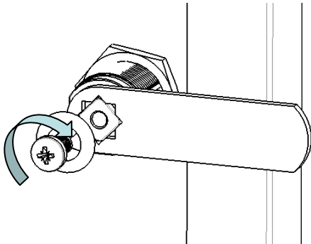
Figure 3. Secure lock with cam, washer & screw. Tighten.
